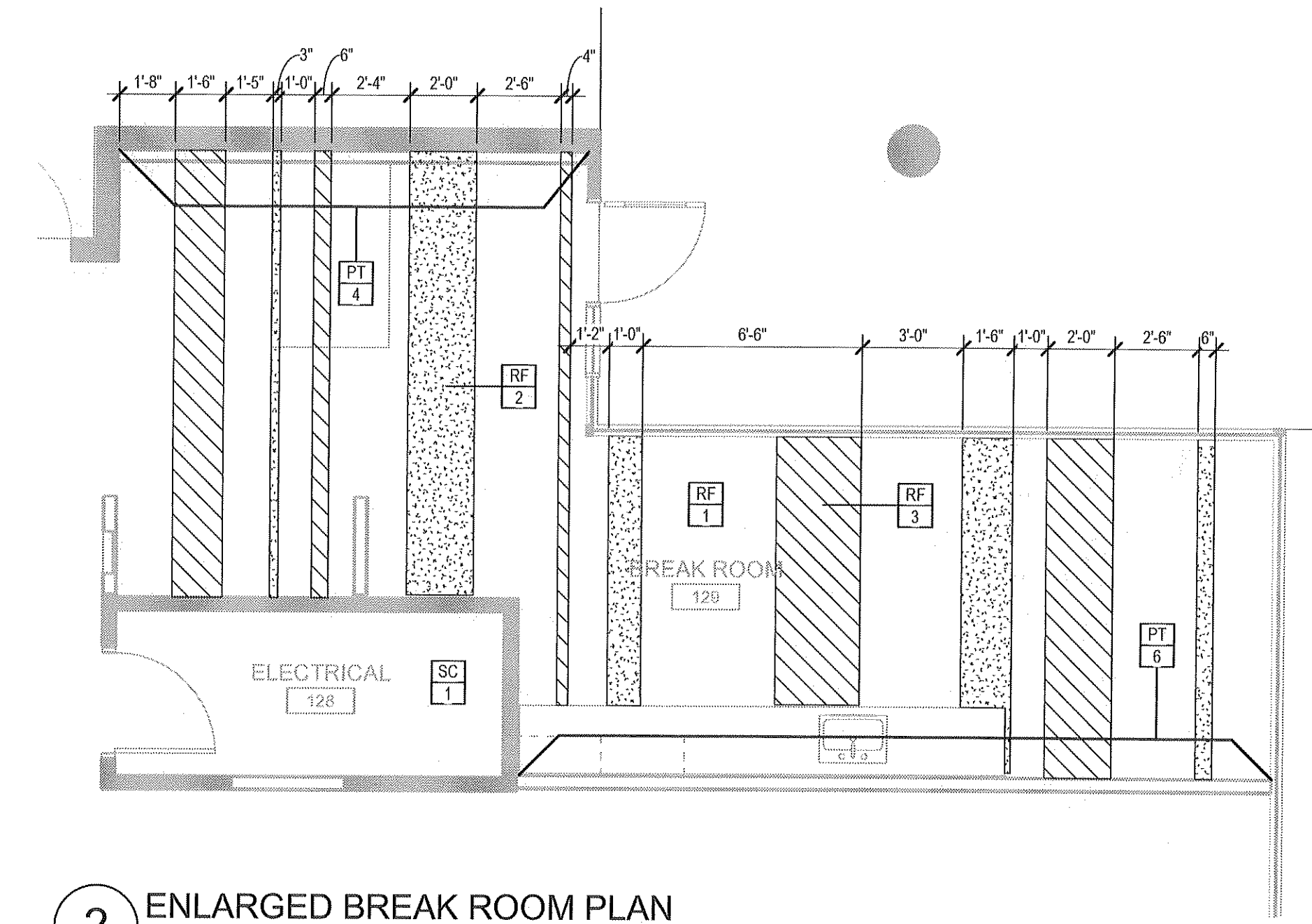
2 ENLARGED BREAK ROOM PLAN 1/4" = 1'-0"
