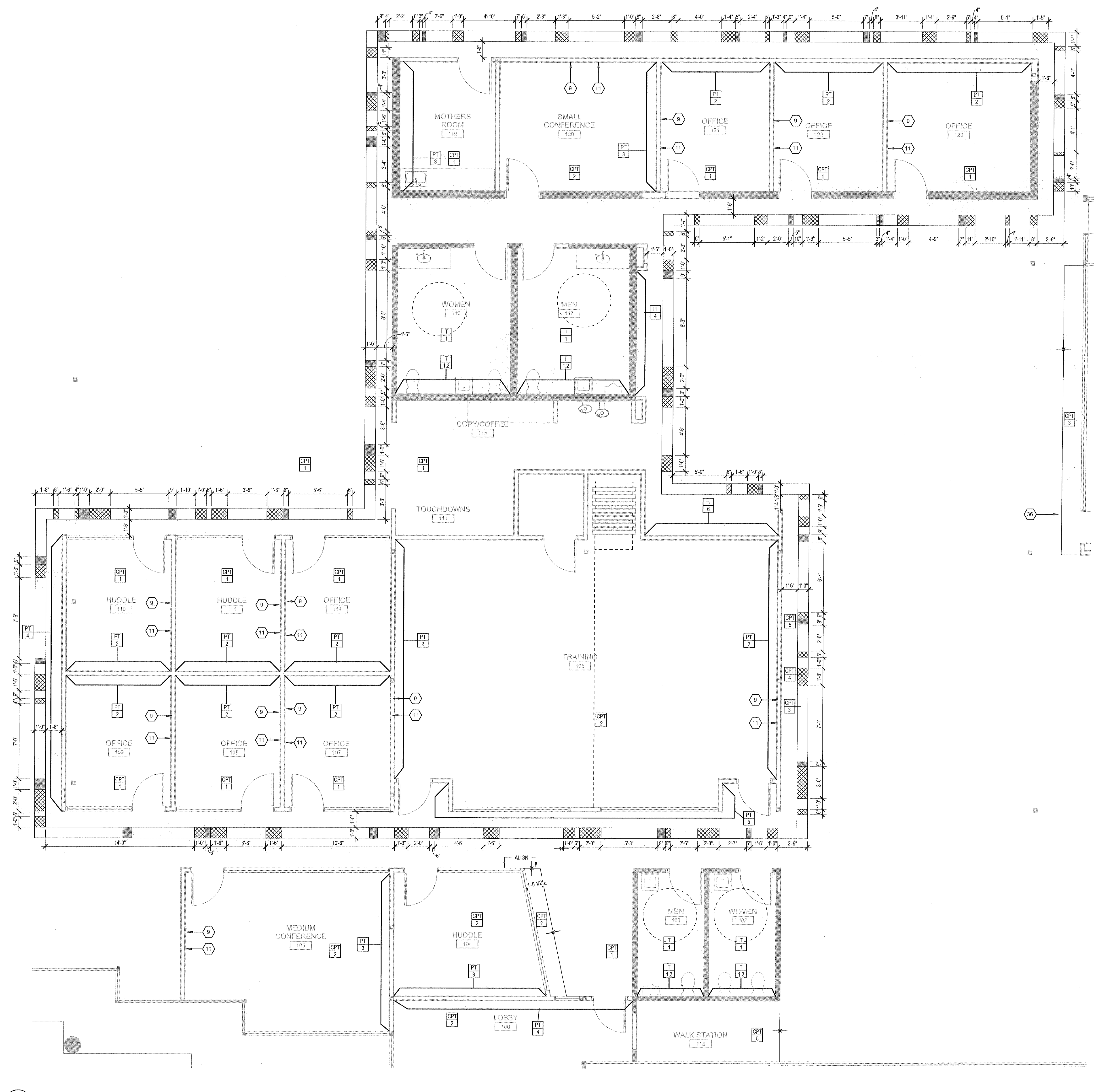
1 ENLARGED LEVEL 1 FINISH PLAN 1/4" = 1'-0"
