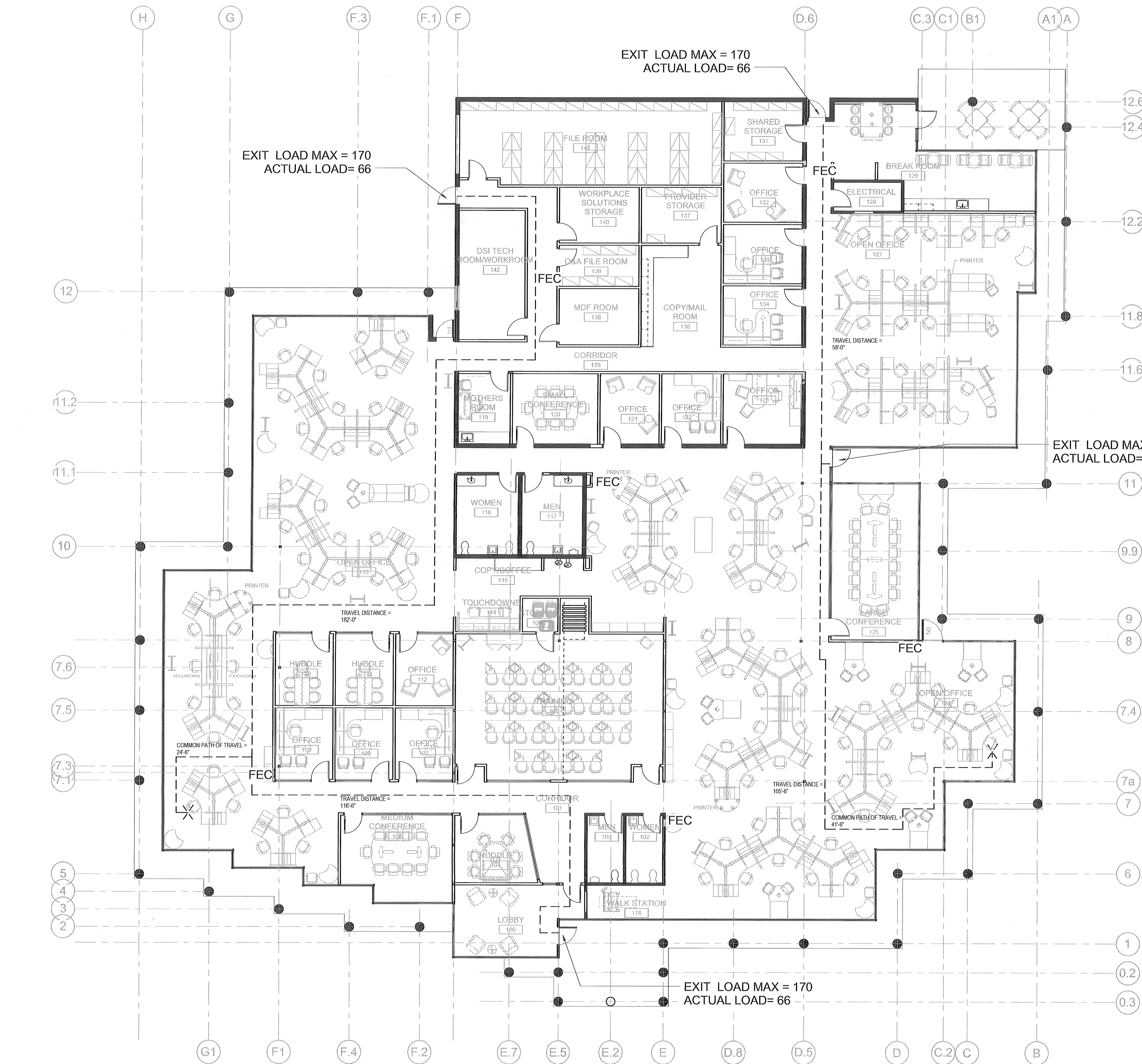
1 LEVEL 1 LIFE SAFETY PLAN 1/8" = 1'-0"
