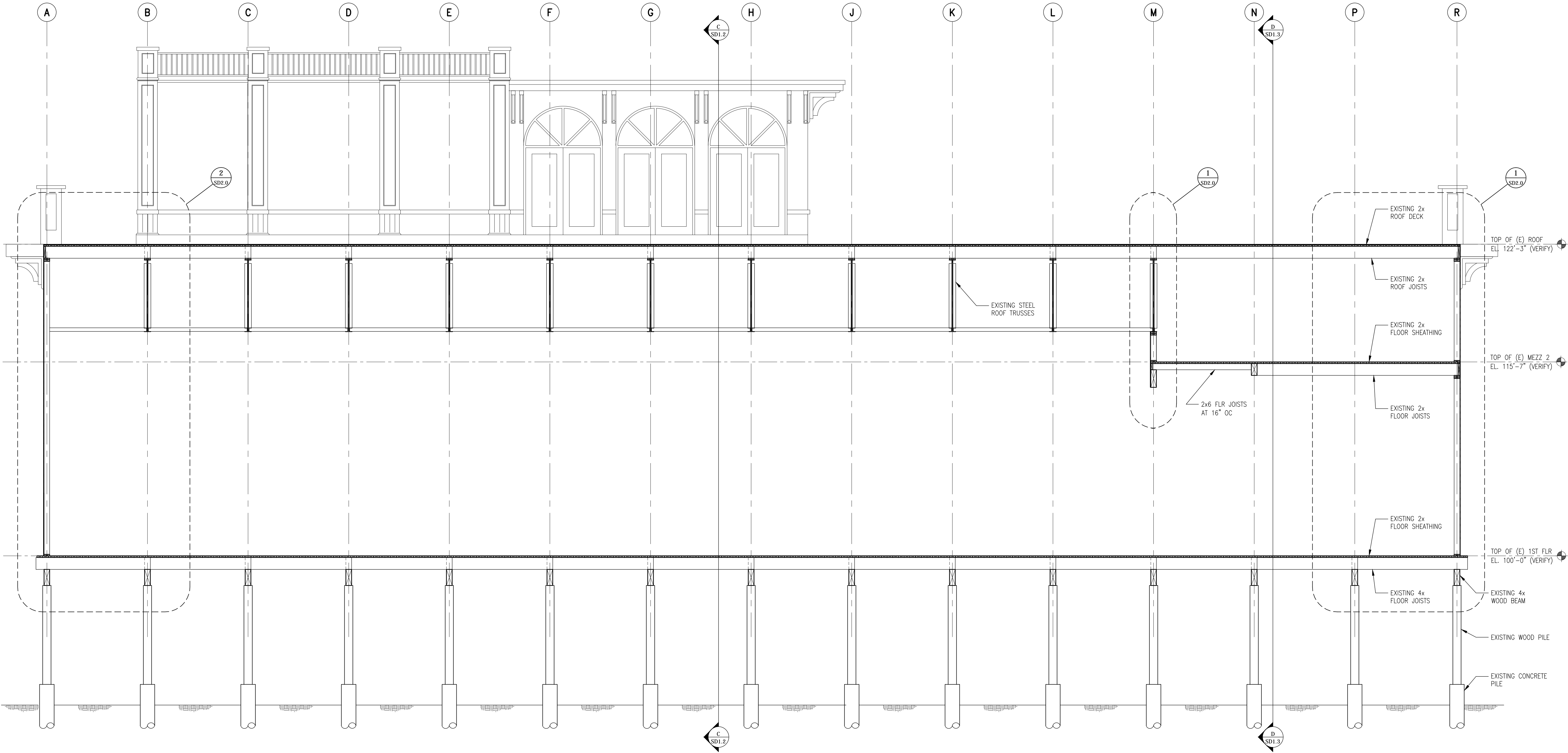
SECTION B-B
