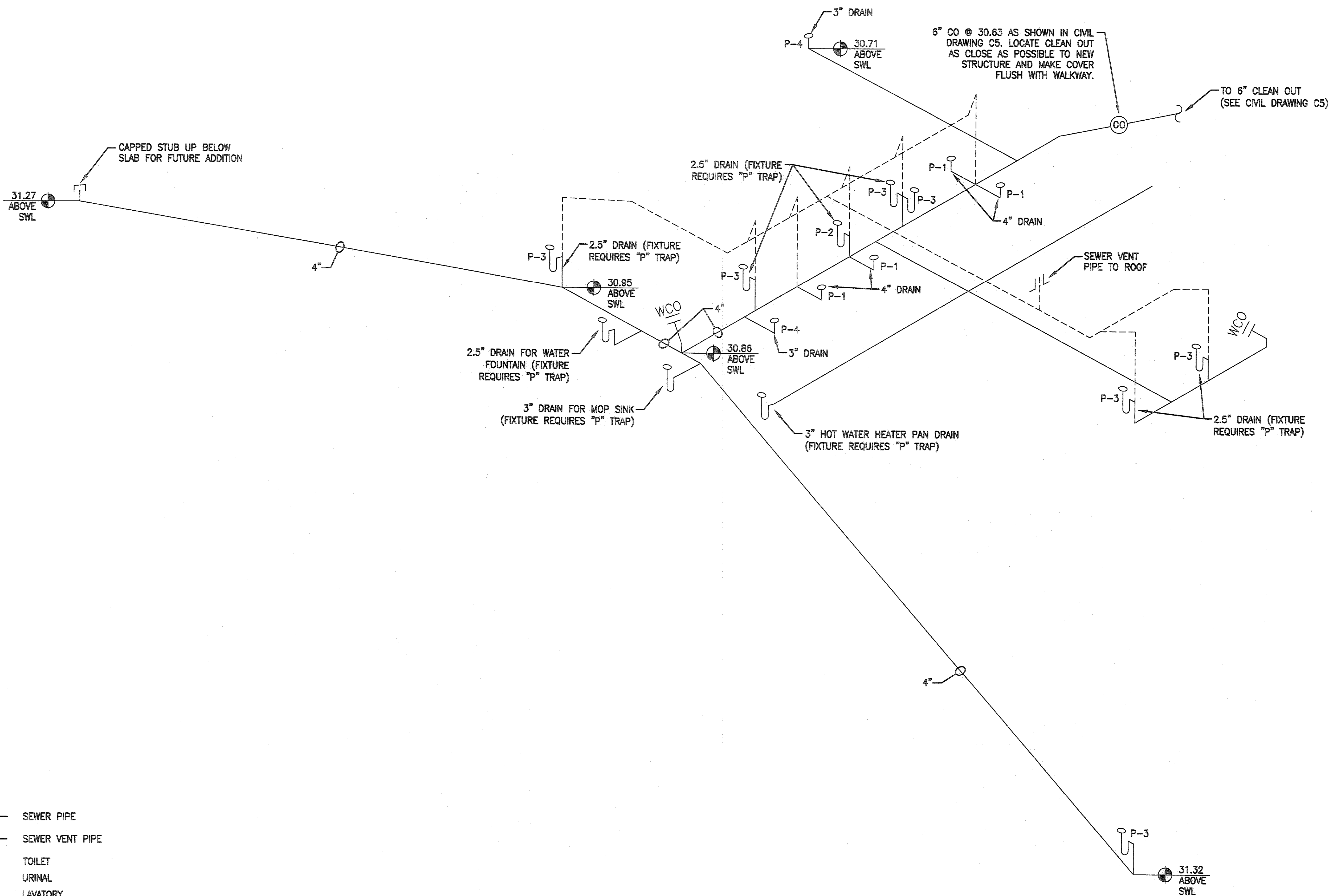
SEWER RISER DIAGRAM NOT TO SCALE
