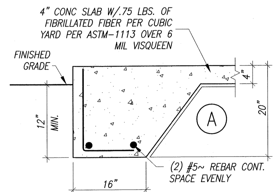
FOOTING DETAIL SCALE: NTS
