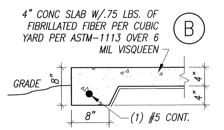
FOOTING DETAIL SCALE: NTS
